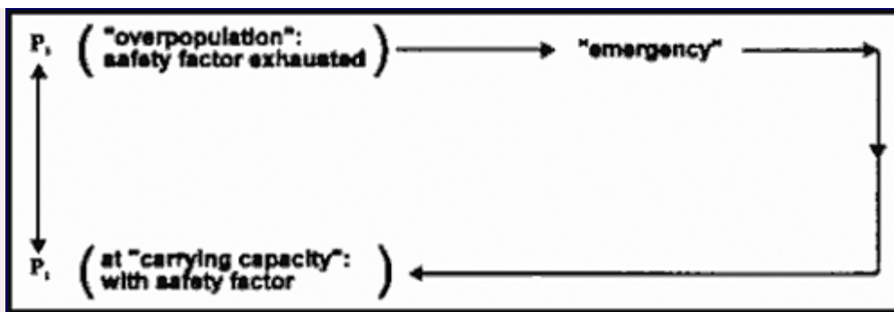
Figure 1. The population cycle of a nation that has no effective, conscious population control, and which receives no aid from the outside. P_2 is greater than P_1 .
