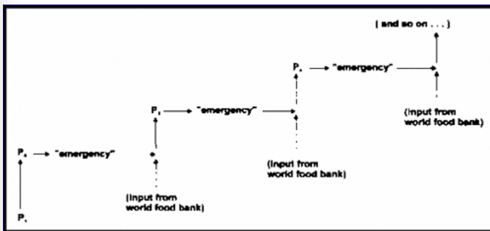
Figure 2. The population escalator. Note that input from a world food bank acts like the pawl of a ratchet, preserving the normal population cycle shown in Figure 1 from being completed. P_{n+1} is greater than P_n , and the absolute magnitude of the "emergencies" escalates. Ultimately the entire system crashes. The crash is not shown, and few can imagine it.
